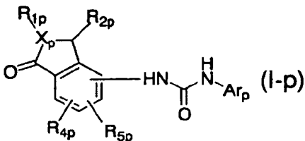
Formula (I-p)
